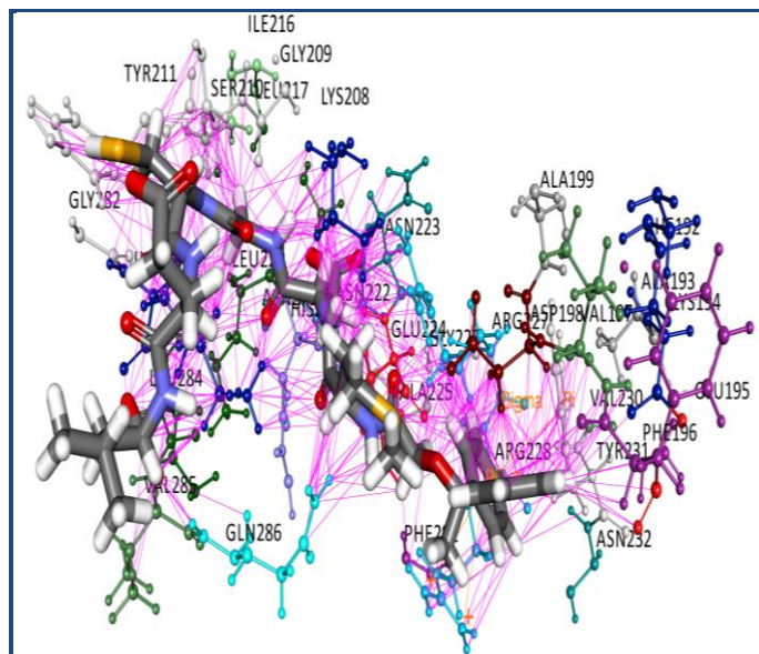
Figure 4: Binding pattern of compound 11 with Wnt5A. The pink lines represent various interactions like electrostatic, van der Waals, steric, hydrogen bonding and hydrophobic interactions that enable energetically favourable binding of the ligand in the cavity.
