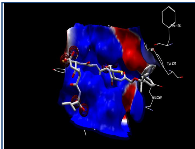
Figure 5: Electrostatic surface of Wnt5a receptor bound with compound 11
