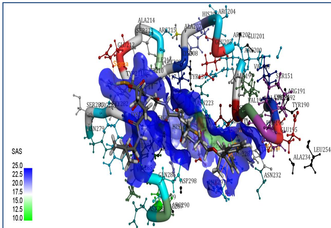
Figure 7: The active site of receptor is shown with solvent accessible surface areas. The accessibility to solvent of the binding site ranges from 10.00 (least solvent accessibility - green shade) to 25.00 (highly solvent accessible -blue shade).
