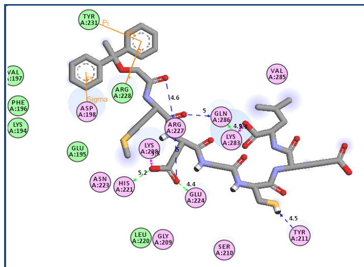
Figure 3: Interactions of compound 11 with Wnt5a protein. Residues circled in green participate in van der Waals interaction with the ligand while residues in pink forms electrostatic interactions. Hydrogen bonds with bond lengths are shown as blue arrows between ligand and residues
