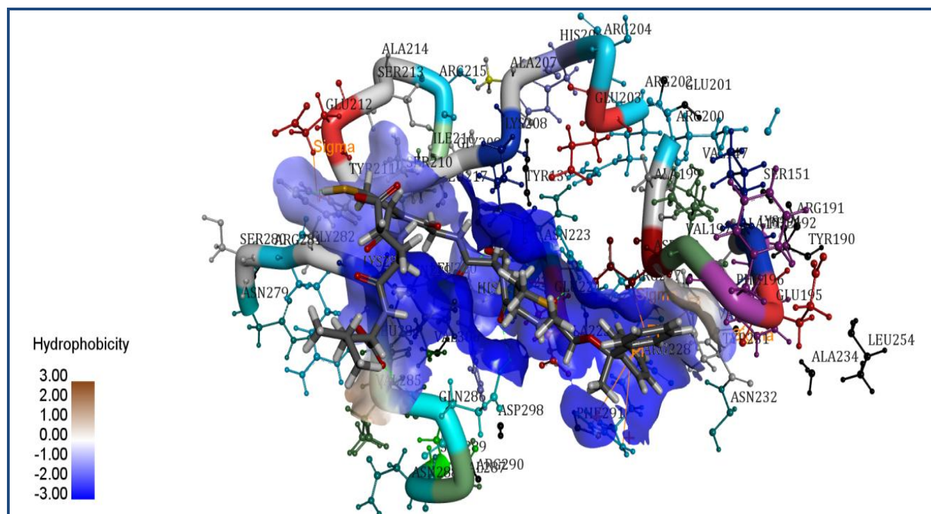
Figure 6: The active site of receptor is shown with hydrophobic intensities. The hydrophobic intensities of the binding site ranges from -3.00 (least hydrophobic area - blue shade) to 3.00 (highly hydrophobic area -brown shade).
