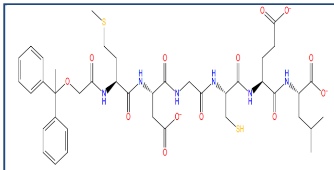
Figure 2: Compound 11. 1,1-diphenylethoxy group attached to N-terminal of hexapeptide (Met-Asp-Gly-Cys-Glu-Leu)
