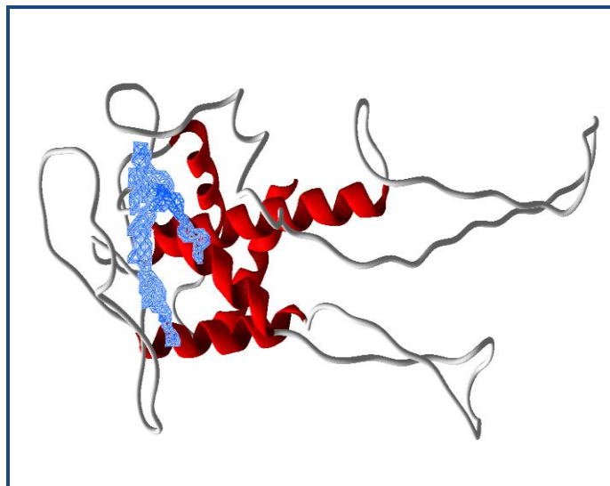
Figure 1: Modeled structure of the Wnt5a protein. Binding site (blue mesh) in the protein was detected using Gaussian Filter enabled DoGSite server
